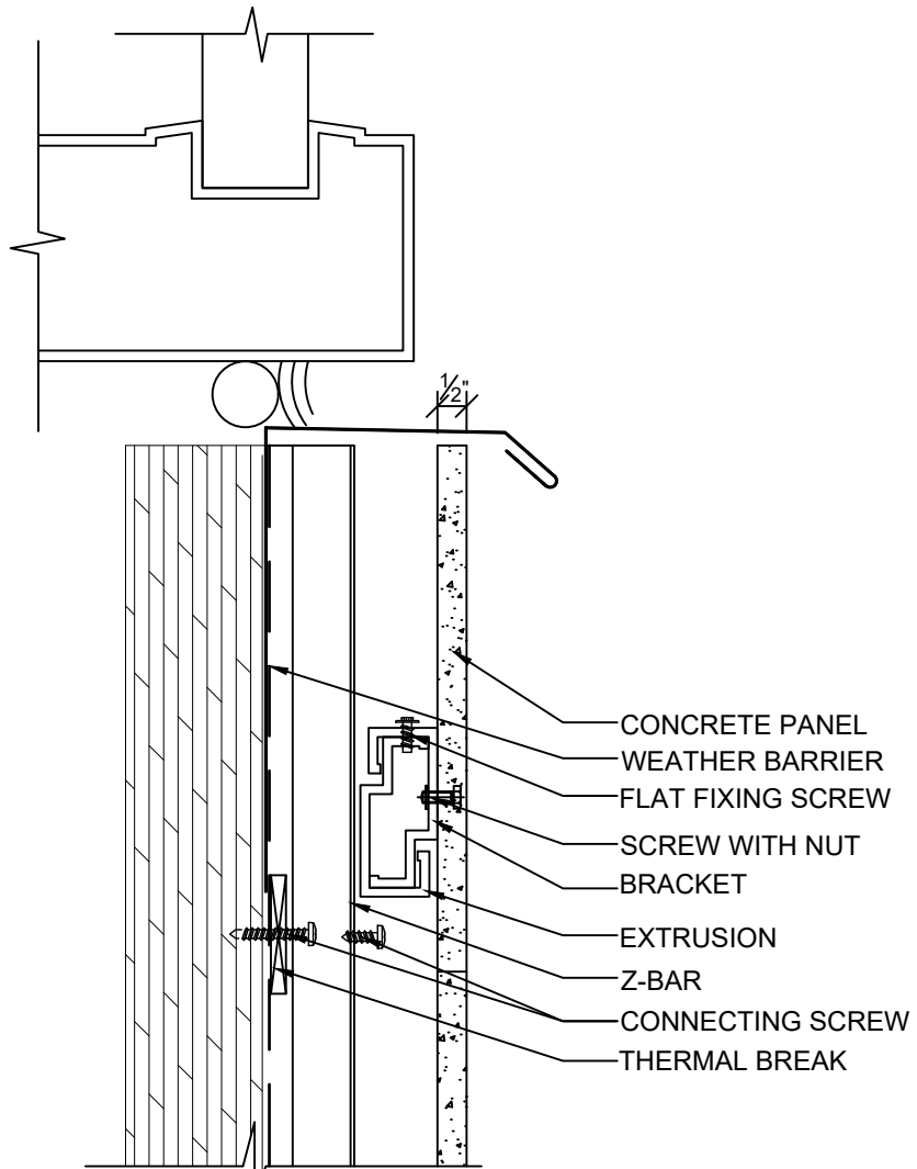
CONCRETE WINDOW Details 3
