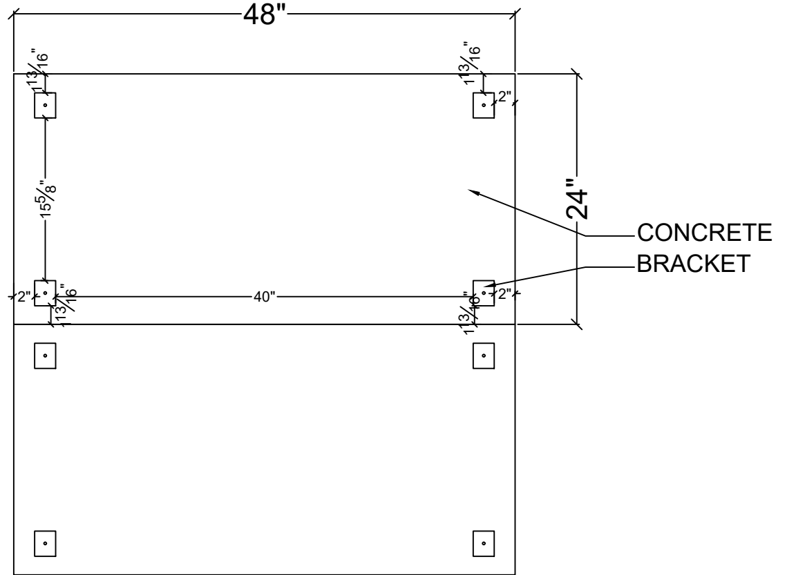
TYPICAL CONCRETE PANEL
