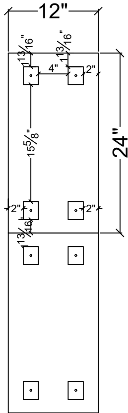
CORNER CONCRETE PANEL
